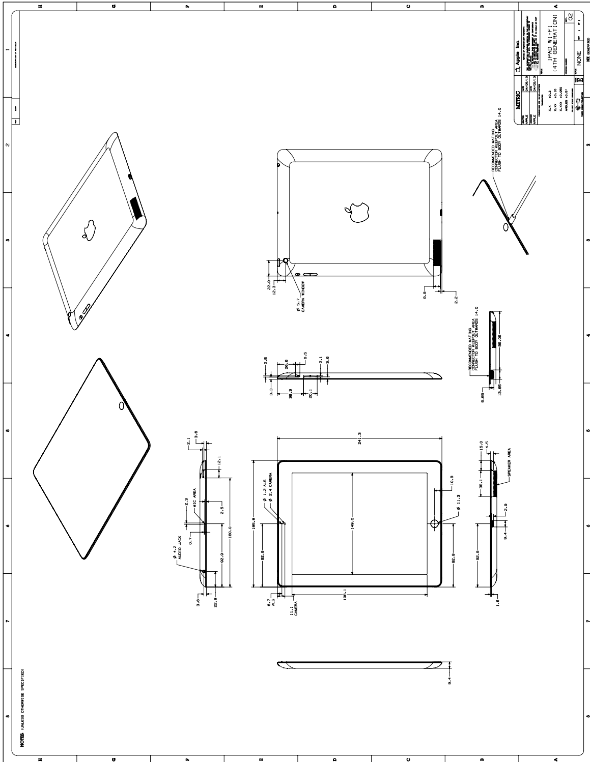
Figure 16-43 iPad (4th generation) with Wi-Fi Dimensional Drawing
